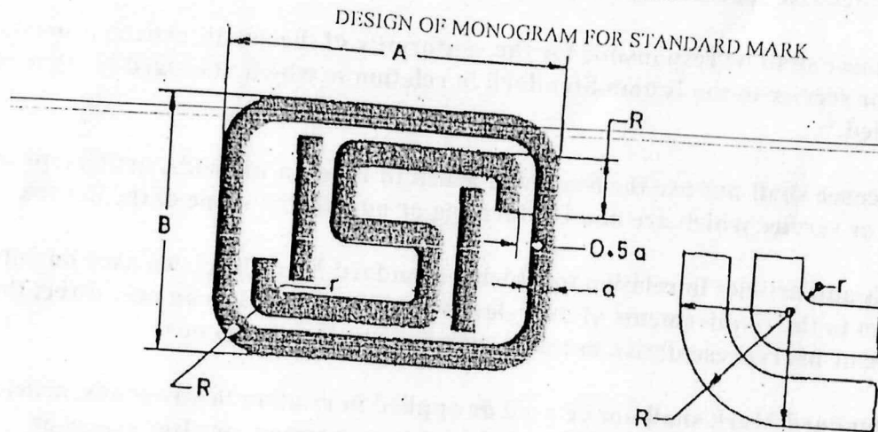
Figure 1 MONOGRAM FOR STANDARD MARK
